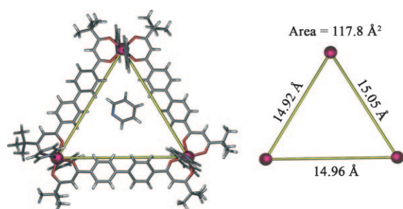
Figure 1. Schematic representation of the crystal structure of [Co_3L_3(py)_6] \cdot 5.55 \text{ py} \cdot 0.6 \text{ H}_2\text{O} . Solvate molecules not shown.
